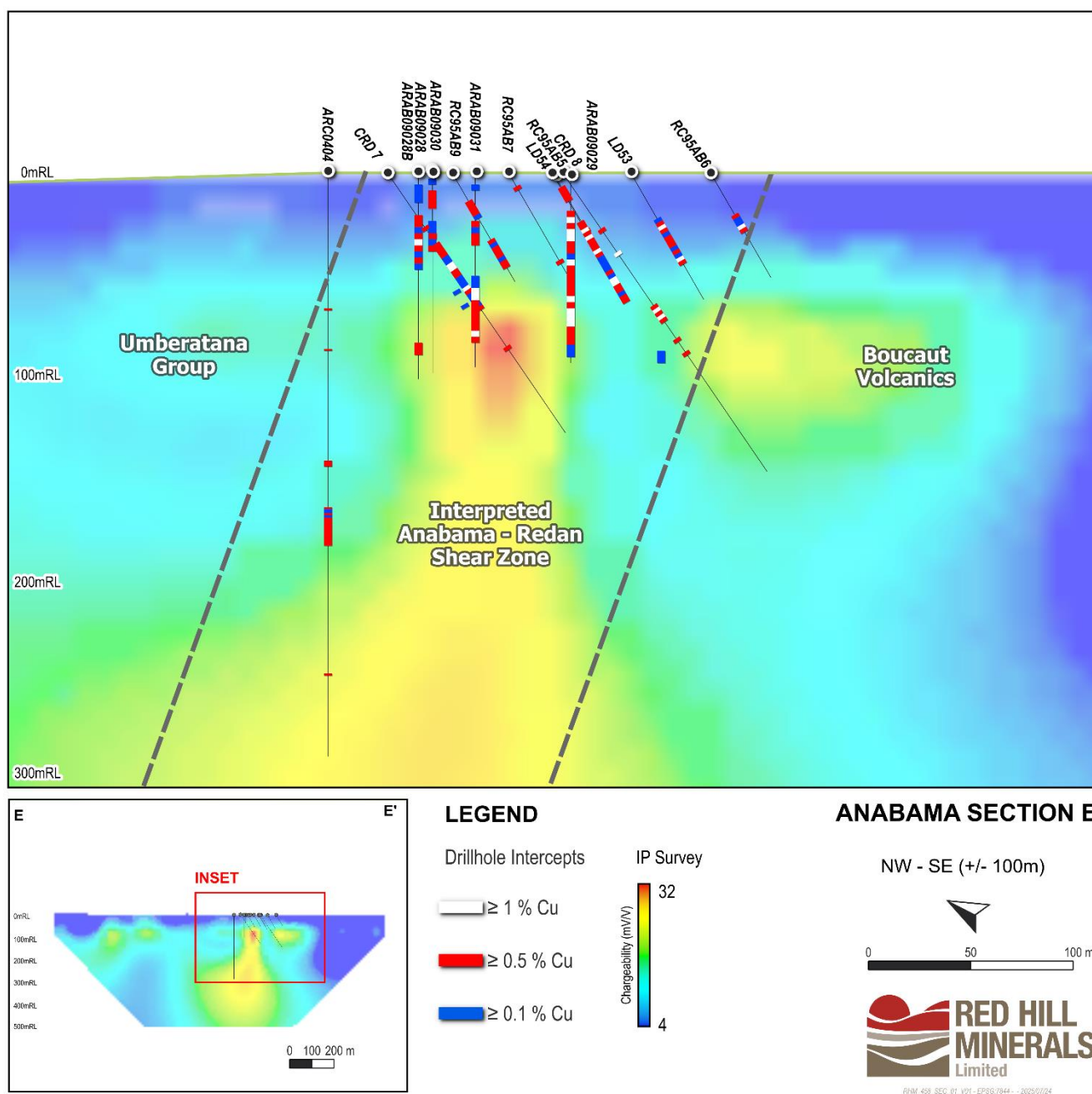
Figure 3: Orientation IP Survey Line E-E' with anomalous copper and gold drilling results 3 over chargeability inversion results and interpreted geology
