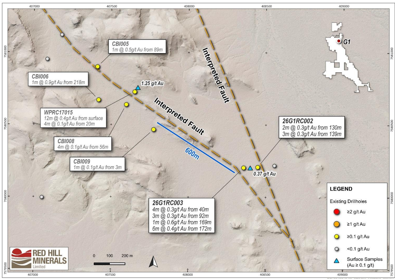
Figure 6: RC drilling hole locations and results at the G1 Target
