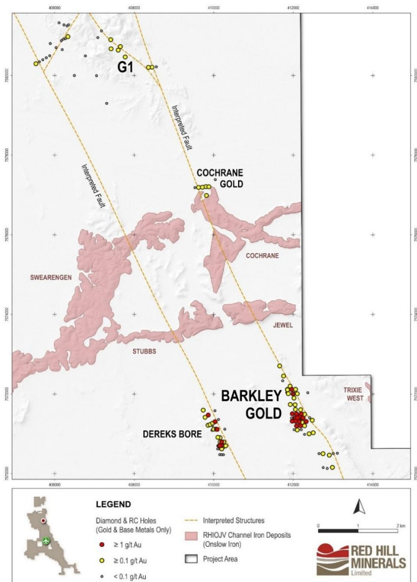
Figure 5: Location plan of the G1 and Barkley Gold Targets. RC and diamond drilling across the regional fault system highlights the widespread strike extent of the gold anomalism.
