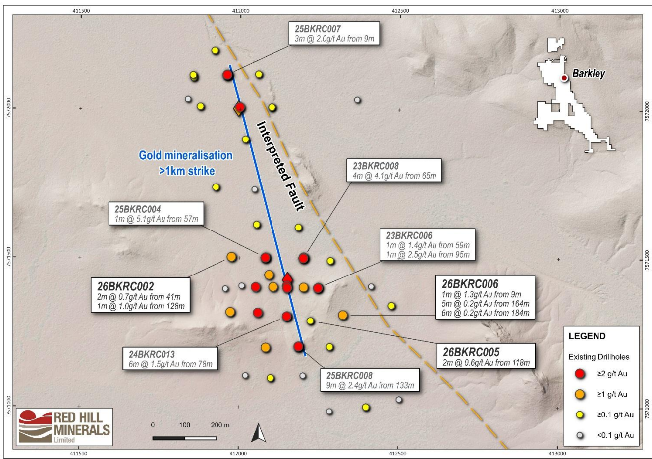
Figure 7: RC drilling hole locations and results at the Barkley Gold Target
