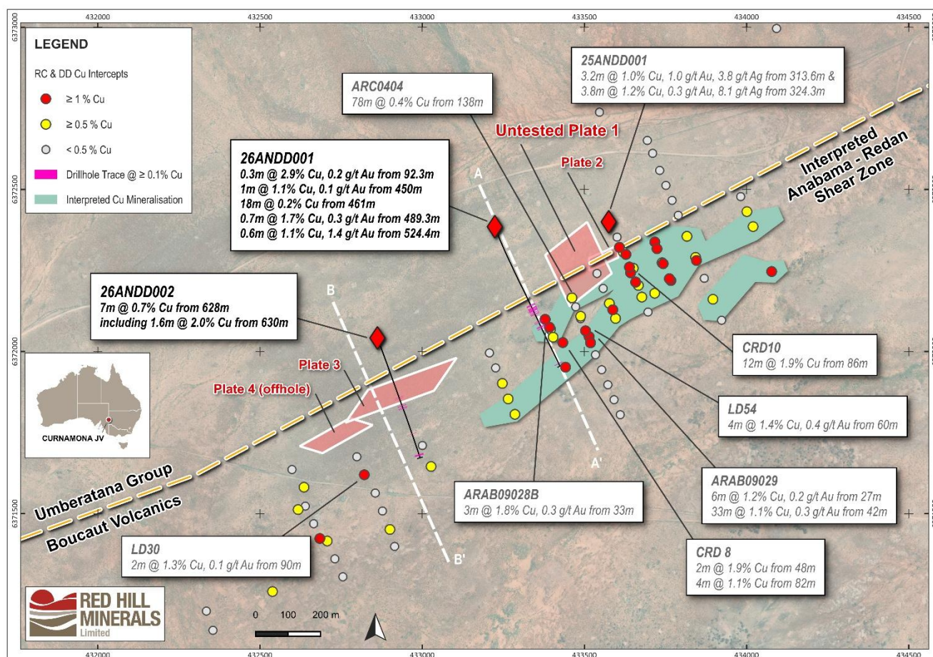
Figure 2: Diamond drill hole locations, assay results, DHEM conductor plates and geological section lines A-A' and B-B' at the Anabama copper-gold target
