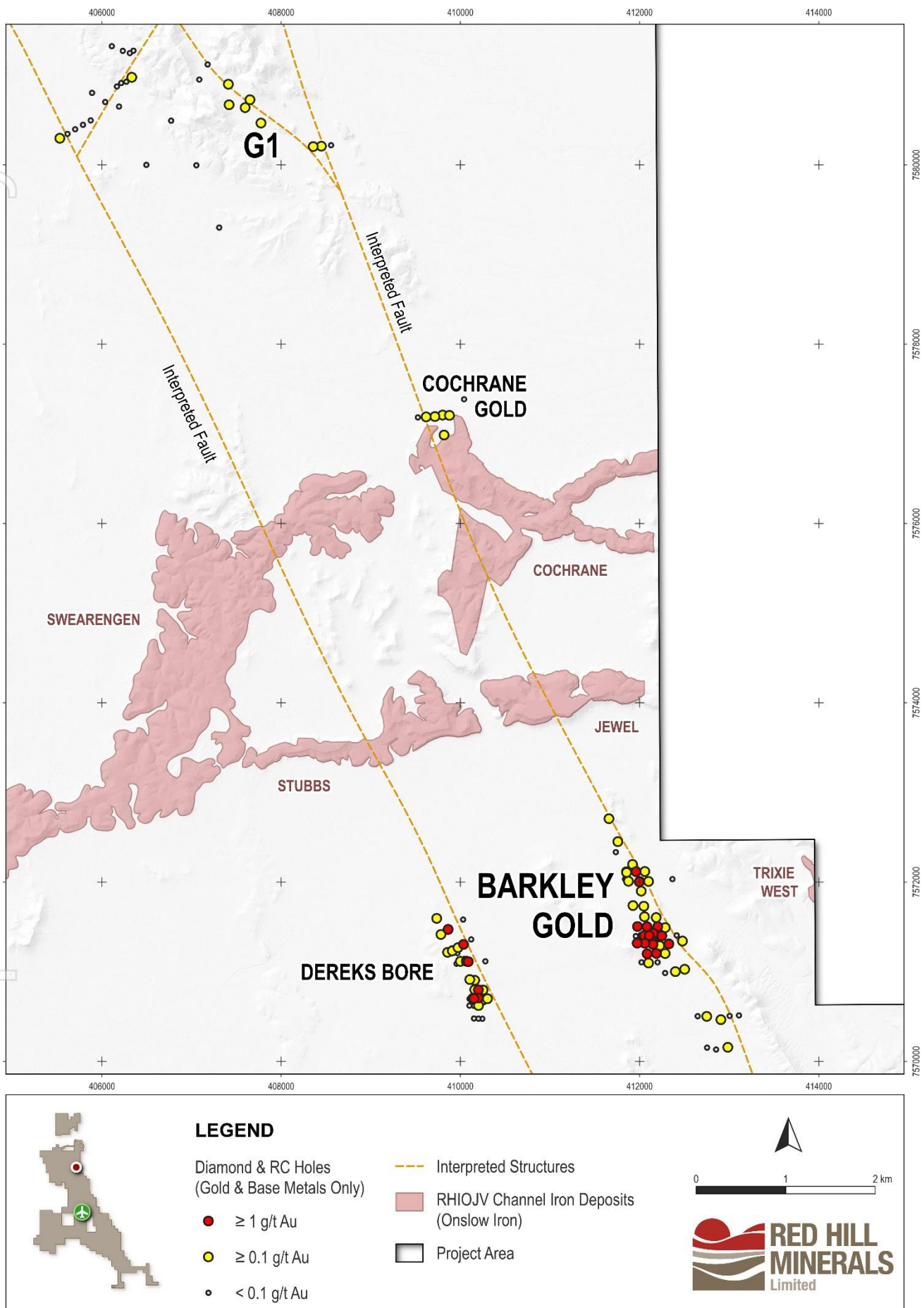
Figure 6: Location plan of the G1 and Barkley Gold Targets. RC and diamond drilling across the regional fault system highlights the widespread strike extent of the gold anomalism.
